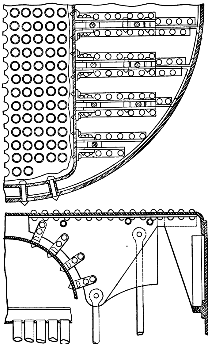
FIG. 106.—STAYING FLAT SURFACES.
